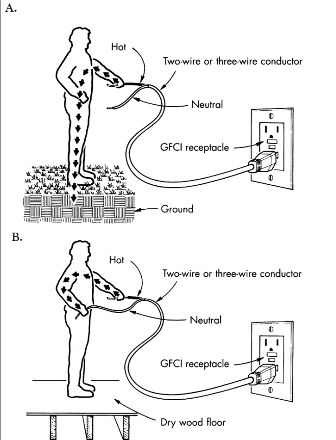
Figure 1. A GFCI trips when it senses a current imbalance, protecting you from shock if you accidentally contact a hot conductor while you are grounded (A). If you come between a black and white conductor and are not grounded, however, a GFCI may not protect you (B), since there will be no current imbalance.
