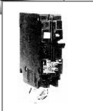
Residential ground-fault circuit interrupters are available in two types. Use receptacle-style GFCIs where possible for convenient resetting at the point of use. GFCI circuit breakers (inset) protect an entire circuit but must be reset at the panel.
