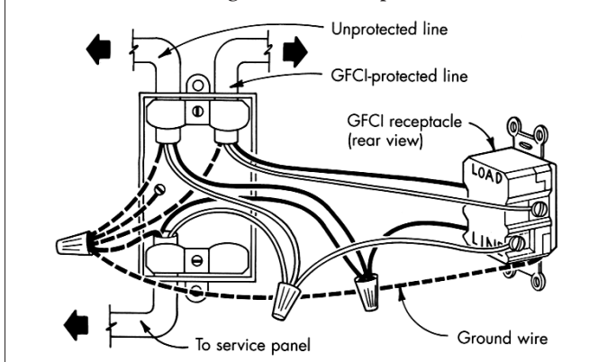
Figure 2. To give ground-fault protection to downstream receptacles, you must wire them off the load side of the GFCI.
