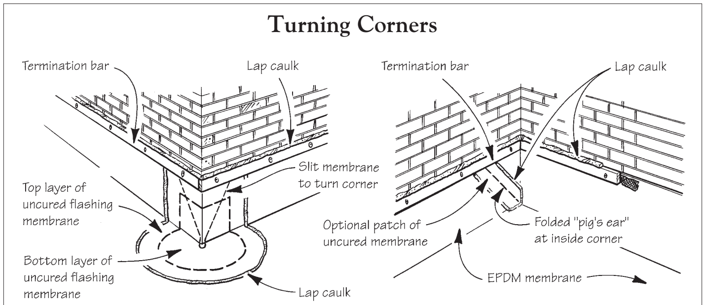
Figure 4. At outside corners, slit the membrane and apply a two-layer patch of uncured flashing membrane (left). Inside corners can either be slit and patched like an outside corner, or folded and secured with a termination bar (right).
