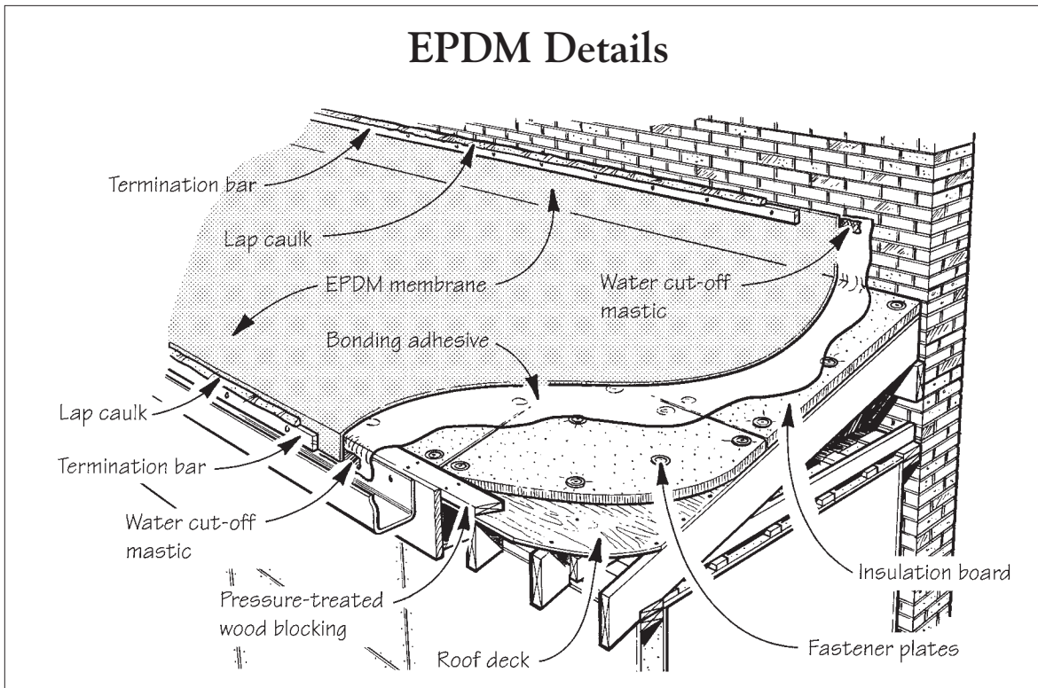
Figure 5. Use aluminum termination bars to secure the edges of an EPDM roof. A special lap caulk protects the top of the termination bar, while a water-block tape or mastic seals the bottom edge of the membrane.
