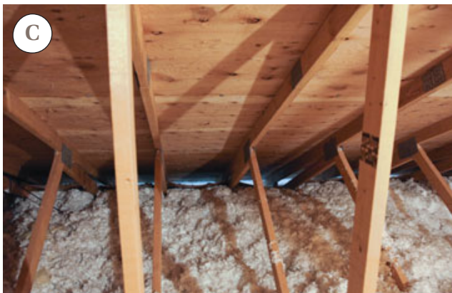
Figure 6. While in theory soffit vents should allow enough cold outdoor air into the attic to prevent snow on the roof from melting, they are often either too small (A) or blocked by insulation (B). Daylight at the eaves is a sign that there is at least some airflow through the soffit vents (C).
