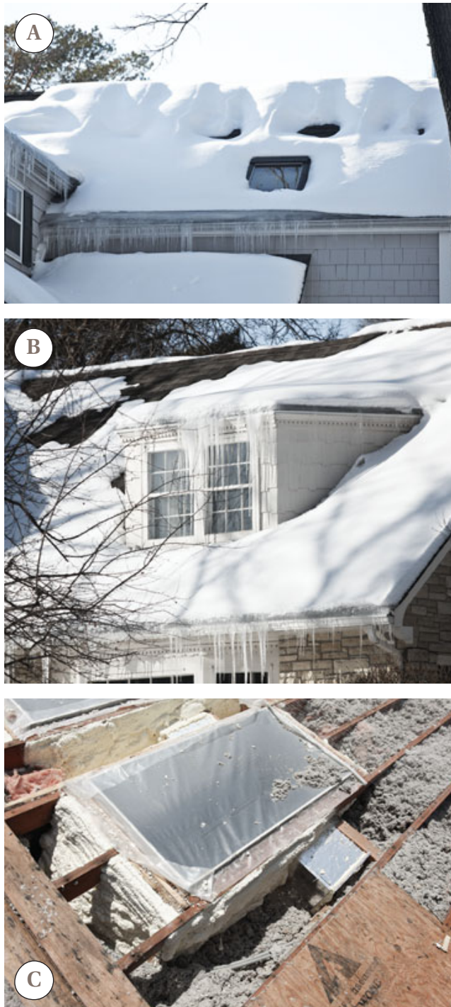
Figure 5. Inadequate insulation (manifested here as lines of snowmelt along the rafters), a narrow, poorly ventilated soffit, and heat loss around the skylight all contributed to ice dams on this house (A). Low-slope roofs, like the one on this shed dormer (B), are commonly plagued with ice dams. In this retrofit job, the author has used two-part spray foam to thoroughly seal and insulate a pair of skylight wells (C).
