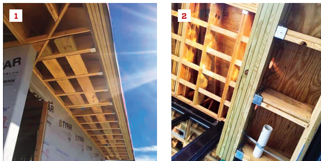
Concealed Gutter Detail
