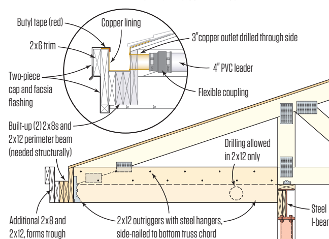
Concealed Gutter Detail
